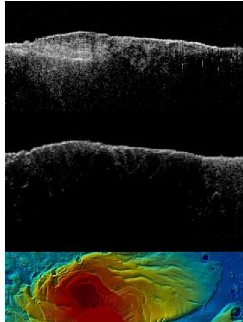
Fig. 2. Comparison between MARSIS real and simulated data. A MARSIS radar section of the Martian subsurface cutting through the Southern polar cap is shown at the top, above a simulation of surface echoes for the same observation. The bottom part of the figure shows a shaded-relief, false colour topographic map of the area produced using the MOLA topographic dataset.
