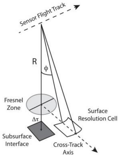
Fig. 1. Diagram illustrating the observation geometry of MARSIS. The area labelled as Fresnel zone is directly under the spacecraft and is the one from which the first echo detected by the radar originates. Both the subsurface interface at nadir and the off-nadir surface resolution cell produce echoes that will reach the radar after the nadir echo.
